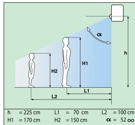
Activation range of PIR detector.
